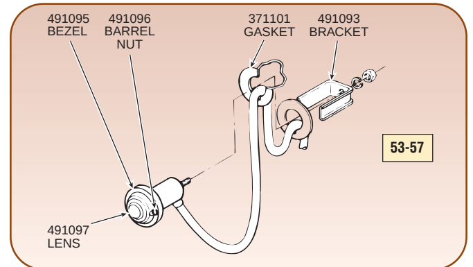
491012 53-54 491085 55-57 Parking Lamp Assembly
